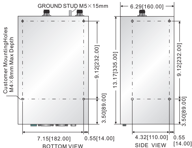
M4:-70kV ~ +70kV 280W Bipolar Output
